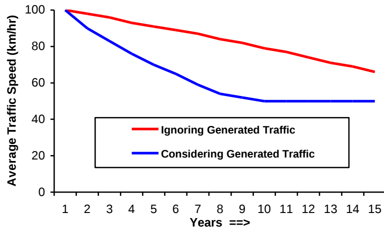
Figure 8 Projected Average Traffic Speeds
