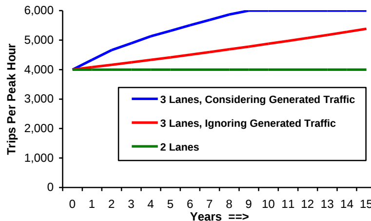
Figure 7 Projected Traffic
